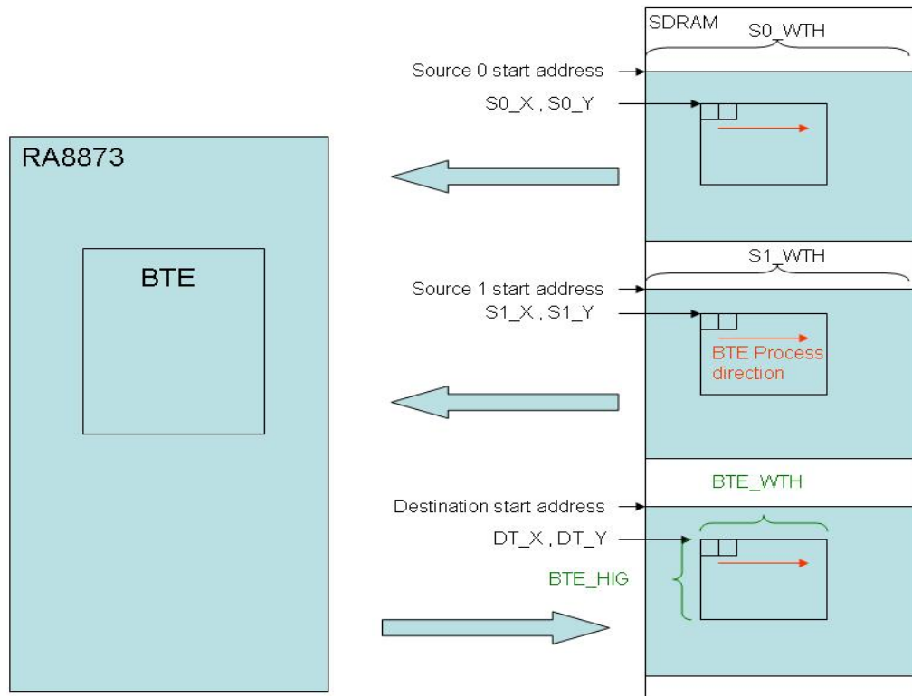
Figure 4-1 : Memory Access of BTE Function
